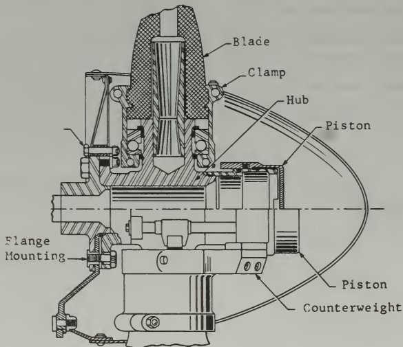
FIGURE 7-12. Constant Speed Prop.
